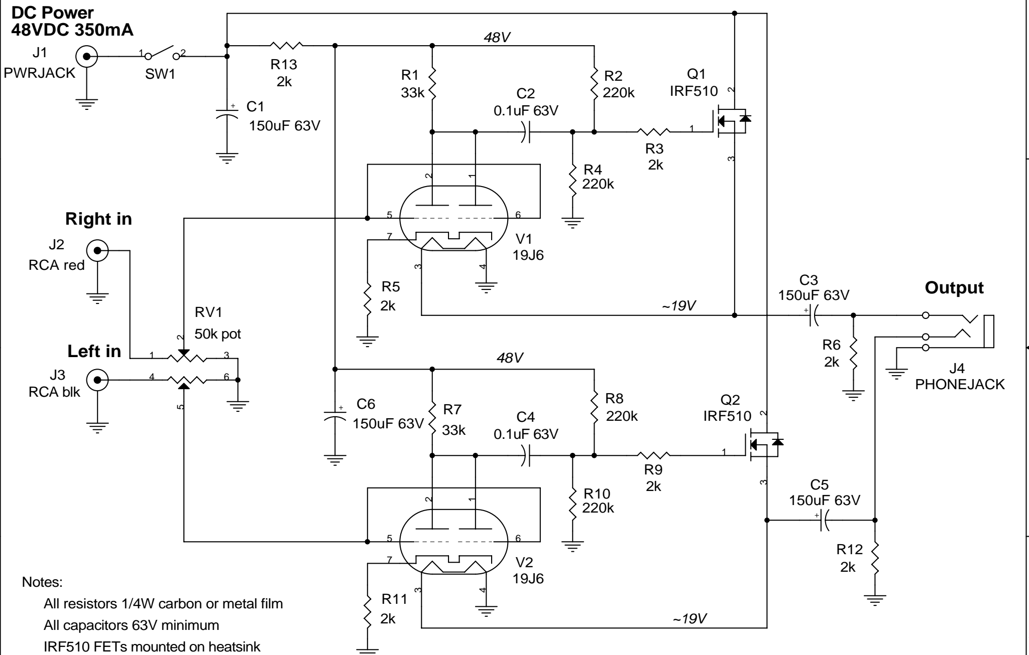
Millett "Starving Student" Hybrid Headphone Amp Pete Millett 2008
