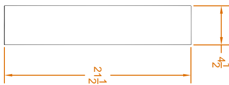
STAND SIDE (MAKE 4)
