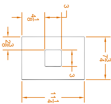
BOTTOM (MAKE 2)
