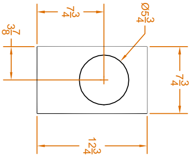
FRONT (MAKE 2)
