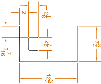
BACK (MAKE 2)
